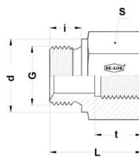
Part No.-MFAE
