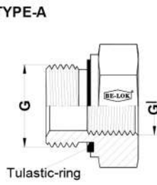
Part No.-MFAB
